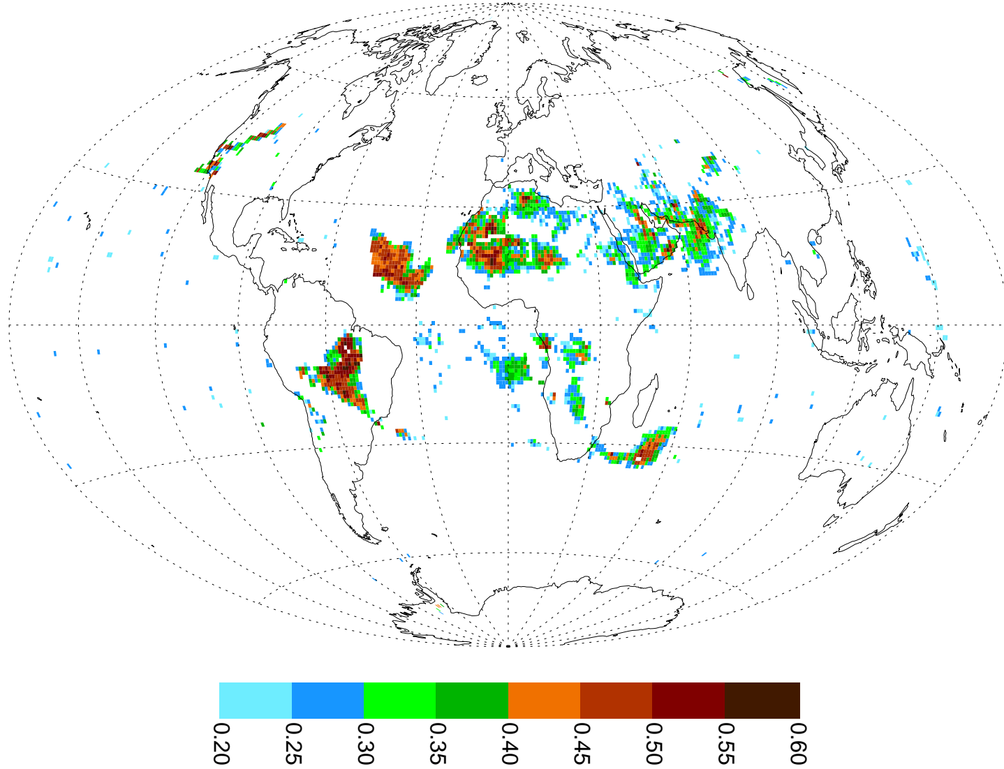
N7/TOMS, Estimated Aerosol Attenuation for 09/03/87
