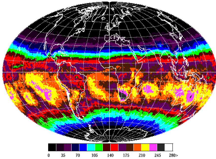
ERYTHEMAL SPECTRAL EXPOSURE (kJ/m 2 ) FOR JANUARY 1992
