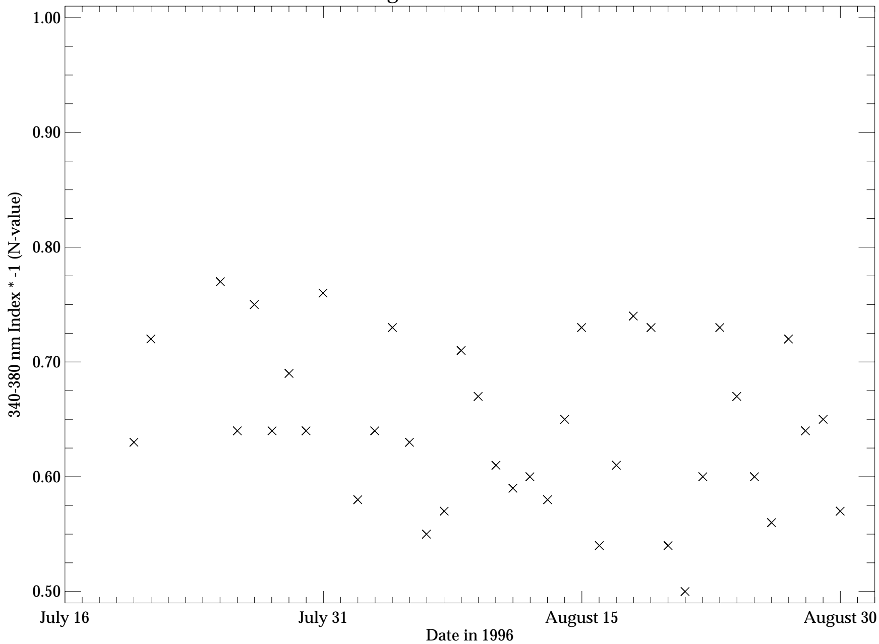
EP/TOMS Non-Absorbing Aerosol Index < -0.5 for 1996 off Va. Beach
