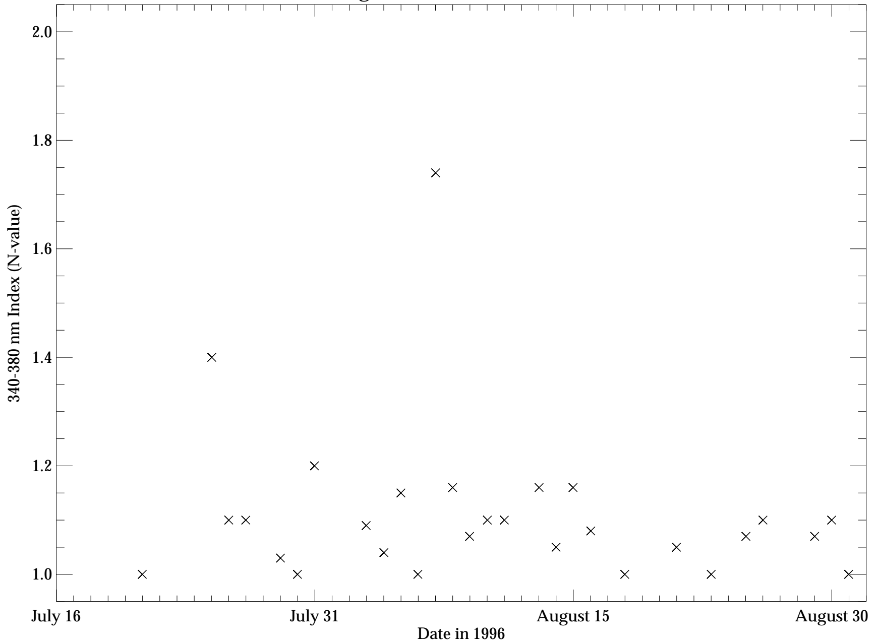
EP/TOMS Absorbing Aerosol Index > 1.0 for 1996 off Va. Beach
