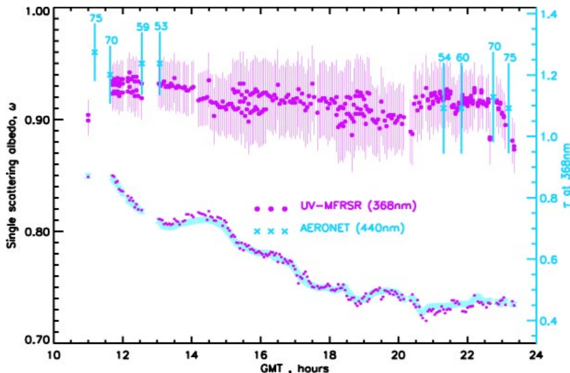
Fig. 2 UV-MFRSR and AERONET \omega retrieval at GSFC on June 24, 2003. The 3-min UV-MFRSR \omega_{368} is shown as small purple spheres, while AERONET \omega_{440} retrievals are shown as large crosses with \pm 0.03 error bars. 27 In addition, \tau_{\text{ext}} at 368 nm is shown for both instruments (same symbols) with right axis scale. The actual solar zenith angle was used in retrieval for each 3-min UV-MFRSR measurement. The UV-MFRSR assumptions were A=0.02 , Brewer-measured total ozone, boundary layer aerosol profile, and AERONET inverted 25 particle size distribution within \pm 30 min of each CIMEL almucantar measurement.
