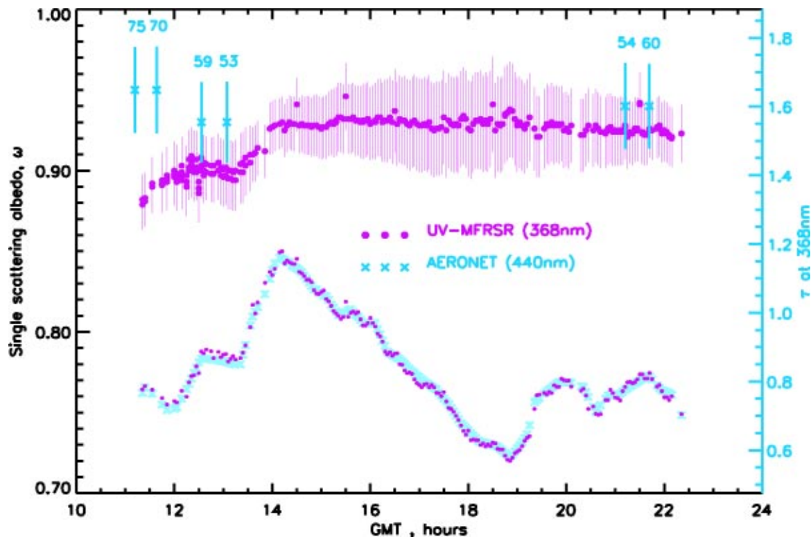
Fig. 1 UV-MFRSR and AERONET single-scattering albedo retrieval at GSFC on June 2, 2003. The 3-min UV-MFRSR retrieved single-scattered albedos at 368 nm are shown as small purple spheres, while AERONET \omega_{440} retrievals at 440 nm are shown as large crosses with \pm 0.03 error bars. 26 The actual solar zenith angle was used in retrieval for each 3-min UV-MFRSR measurement. The UV-MFRSR assumptions were surface albedo of 0.02, Brewer-measured total ozone, and boundary layer aerosol profile and Dubovik and King 25 inverted particle size distribution within \pm 30 min of each CIMEL almucantar measurement.
