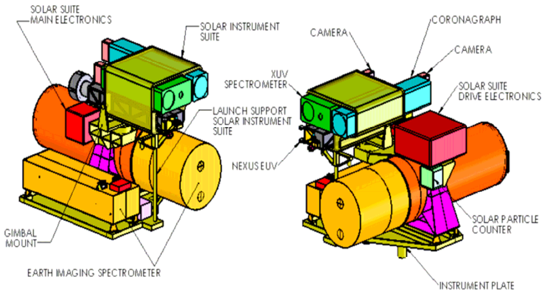
Figure 7 Janus observing system block diagram showing both solar and earth observing telescopes. Solar package points independently from the Earth observing telescopes.
