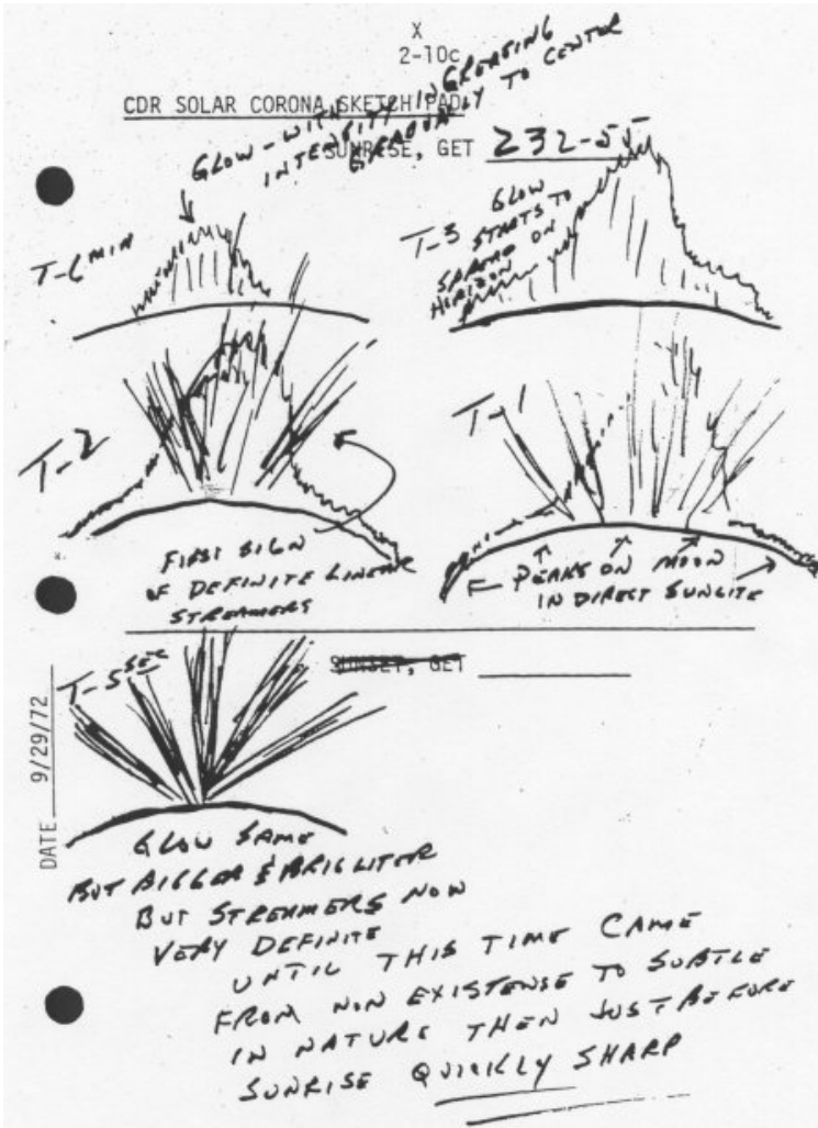
Figure 9 Observations of electrostatic suspension of dust by the Apollo astronauts.
