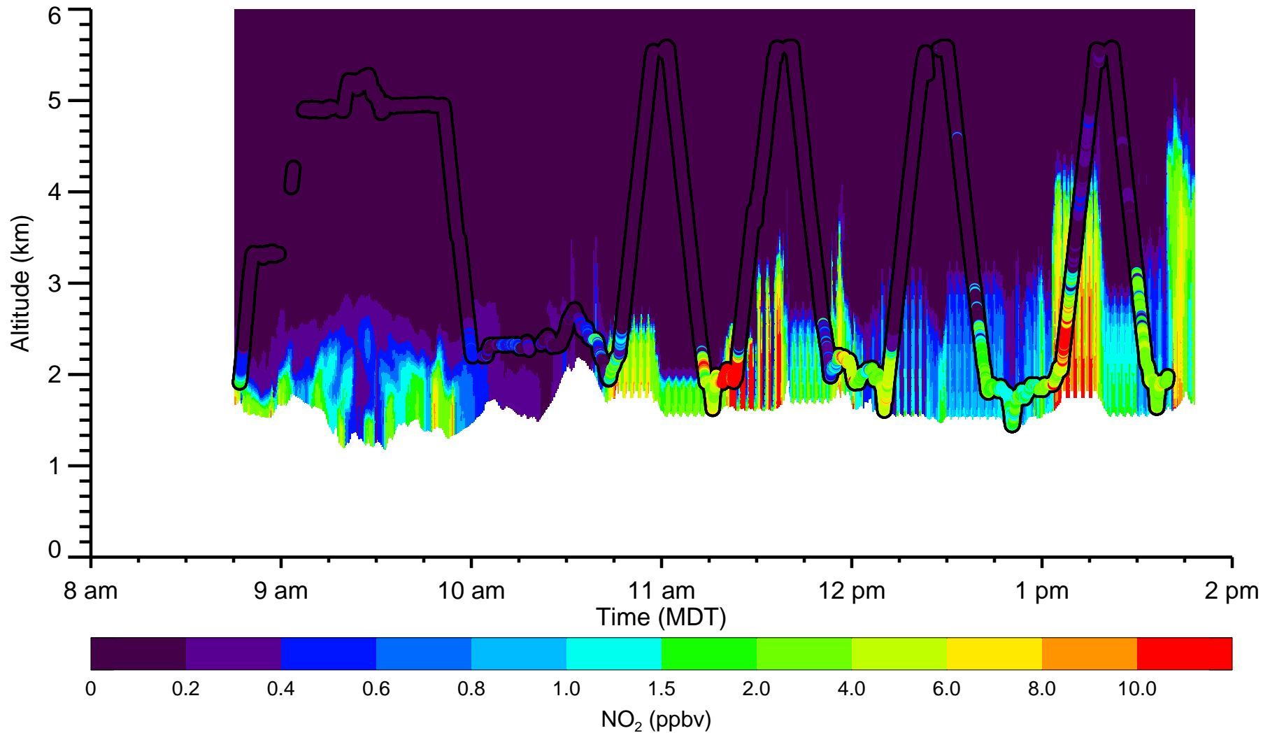
Flight #14 08/08/2014 WRFChem NO 2 and Weinheimer NO 2
