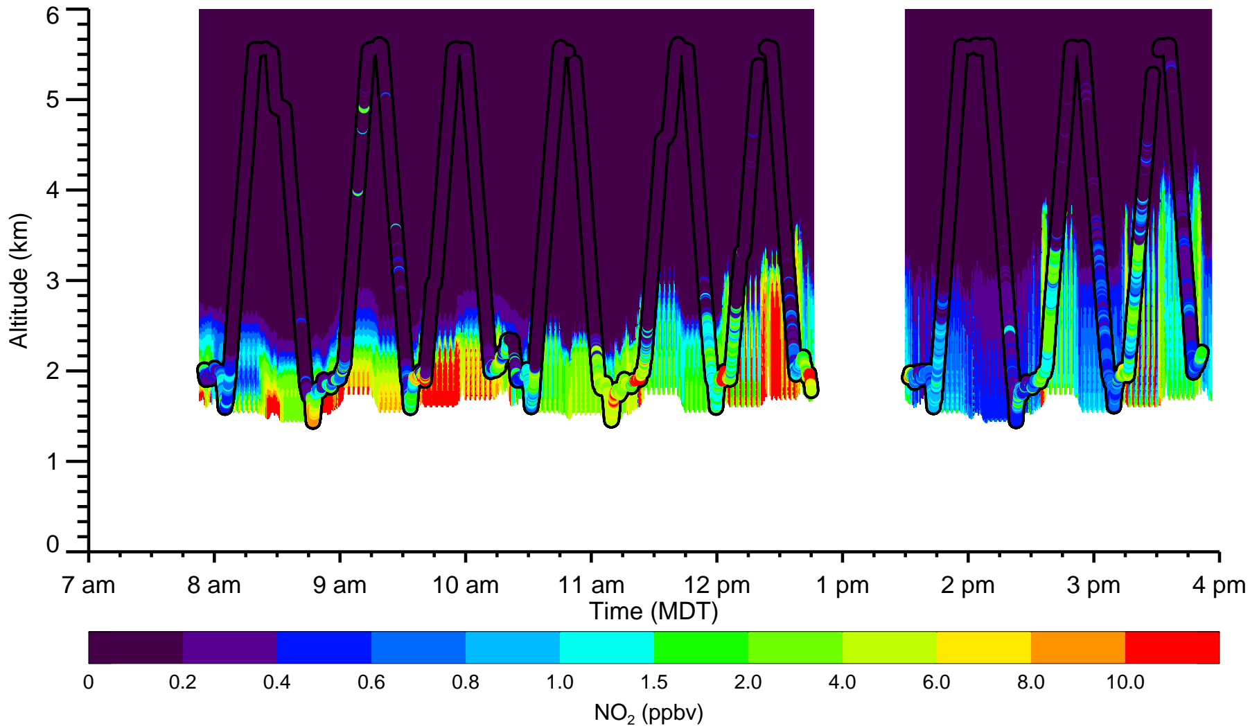
Flight #10 08/02/2014 WRFChem NO 2 and Weinheimer NO 2
