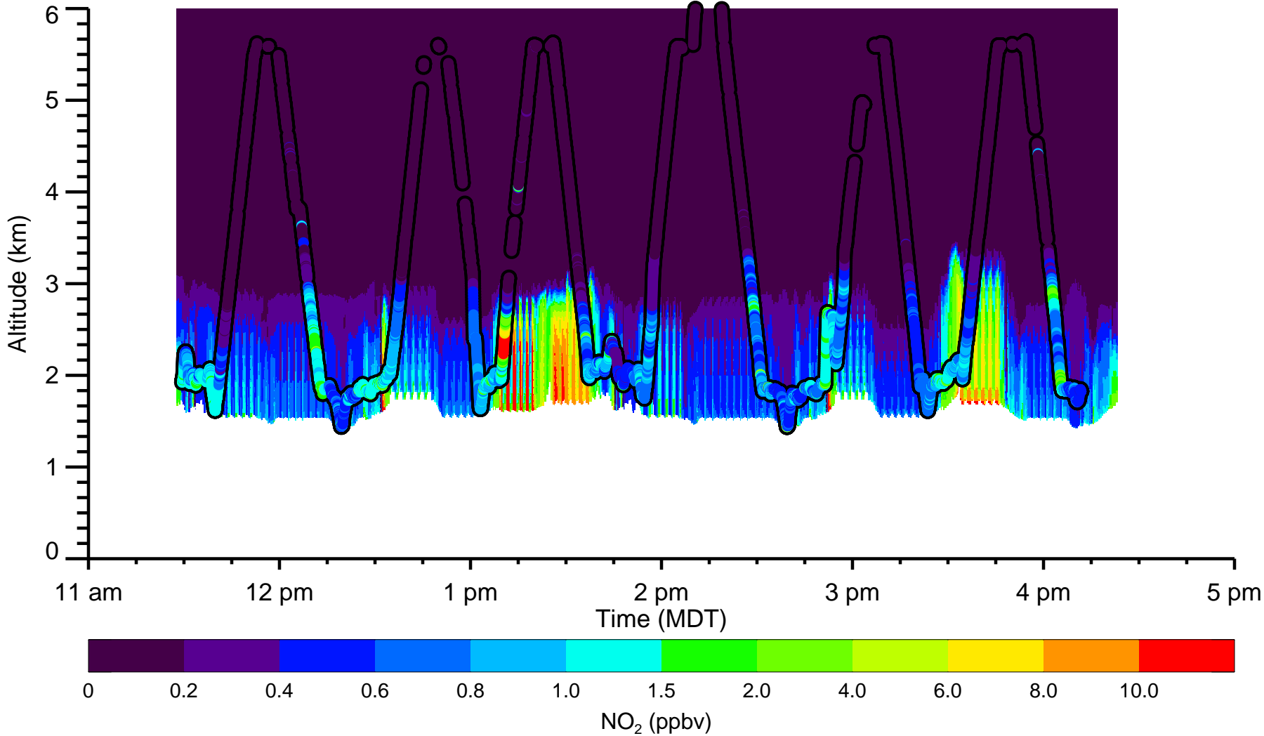
Flight #6 07/27/2014 WRFChem NO 2 and Weinheimer NO 2
