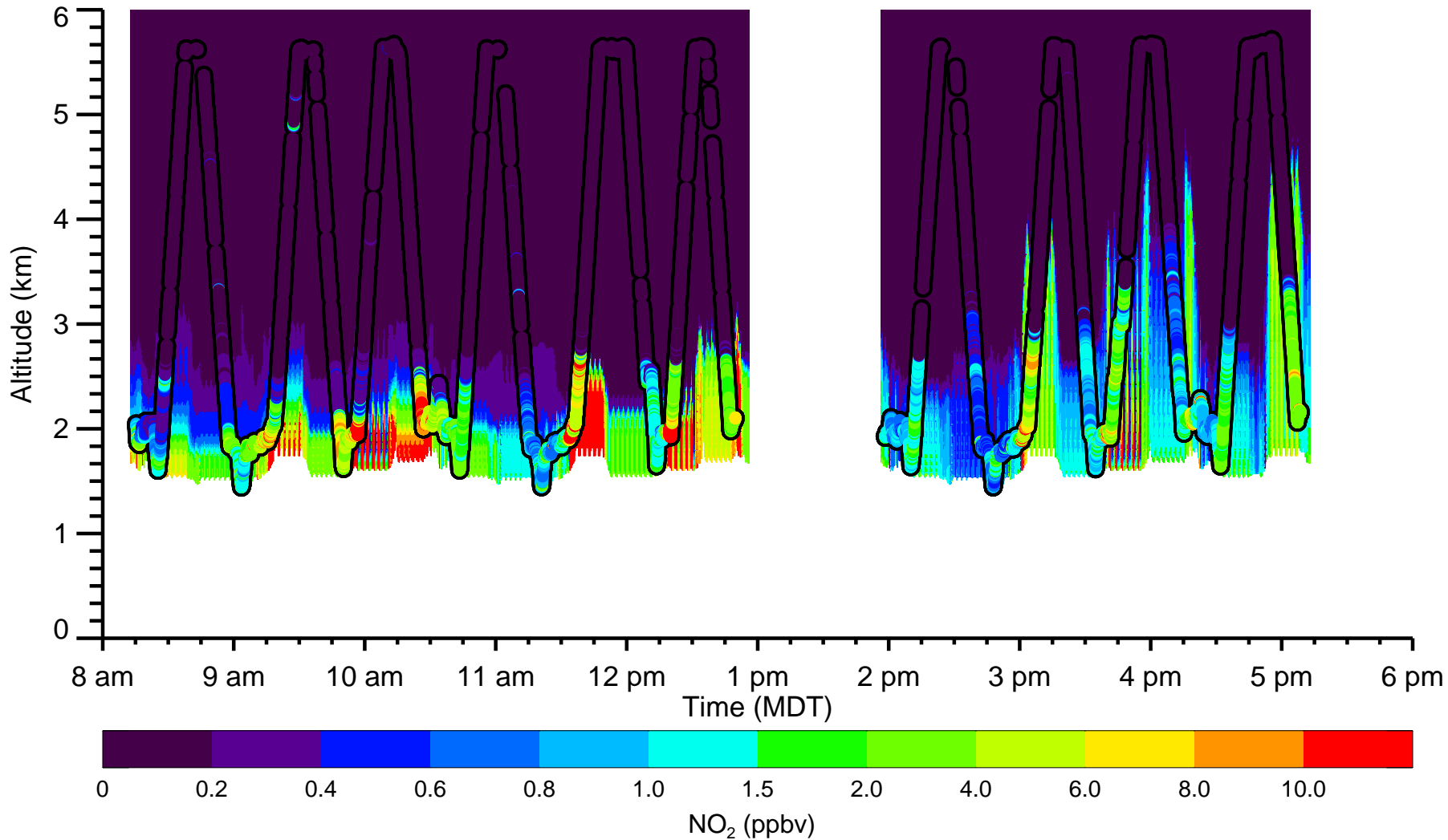
Flight #4 07/22/2014 WRFChem NO 2 and Weinheimer NO 2
