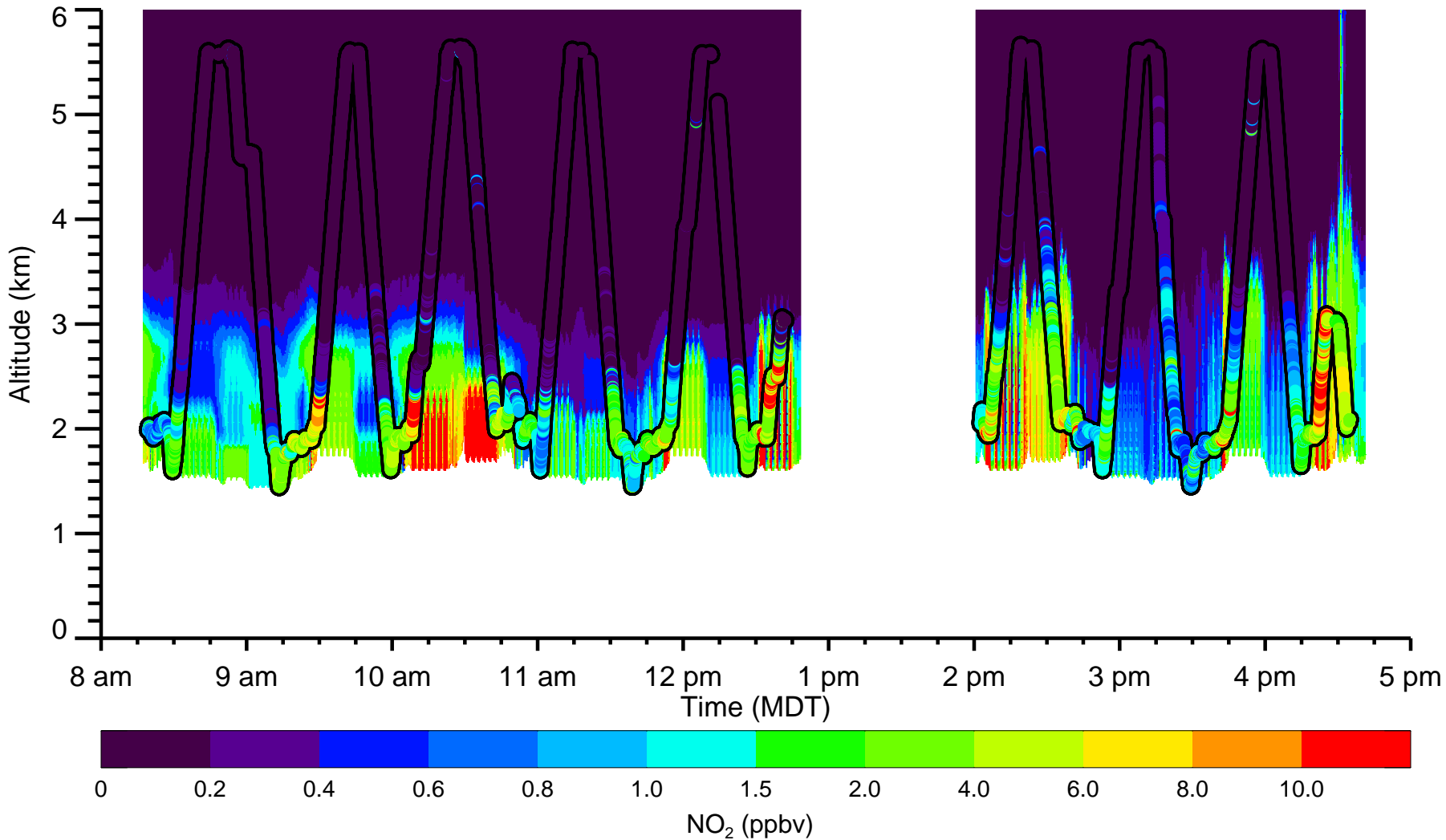
Flight #7 07/28/2014 WRFChem NO 2 and Weinheimer NO 2
