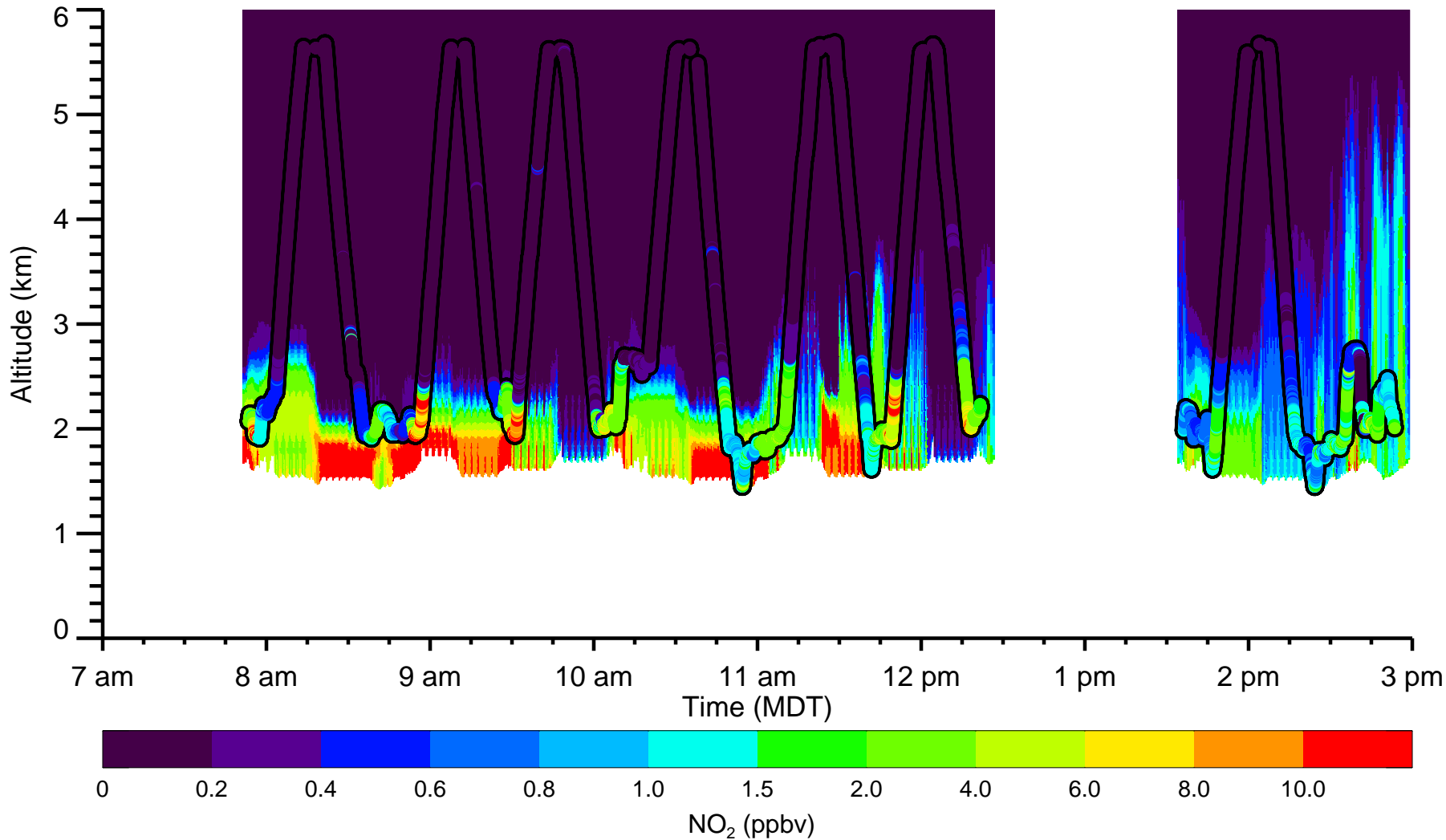
Flight #5 07/23/2014 WRFChem NO 2 and Weinheimer NO 2
