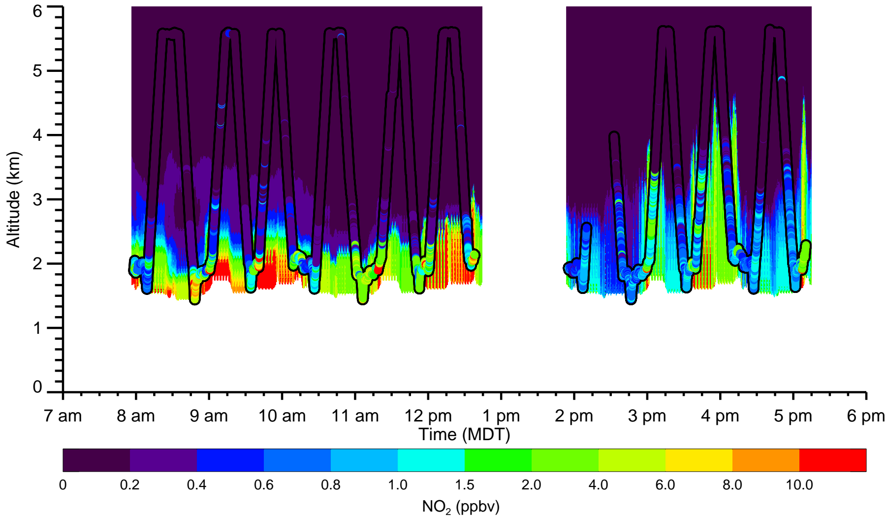
Flight #11 08/03/2014 WRFChem NO 2 and Weinheimer NO 2
