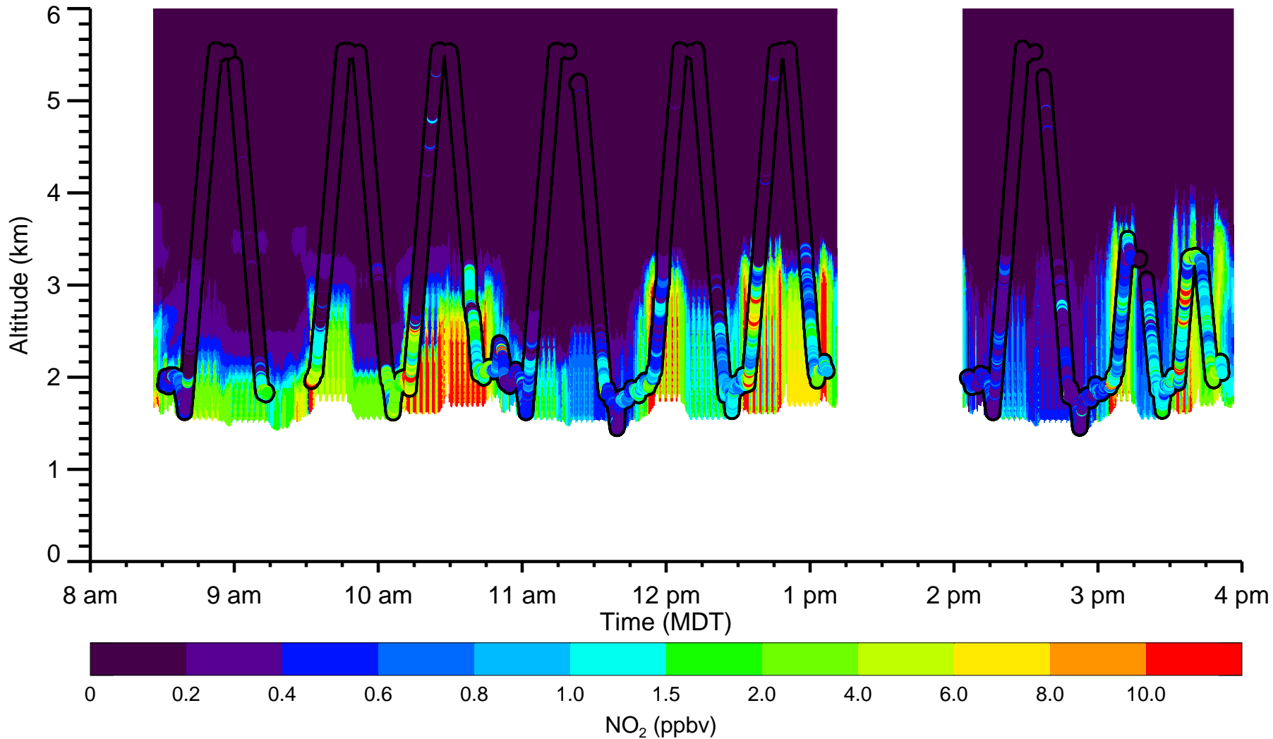
Flight #15 08/10/2014 WRFChem NO 2 and Weinheimer NO 2
