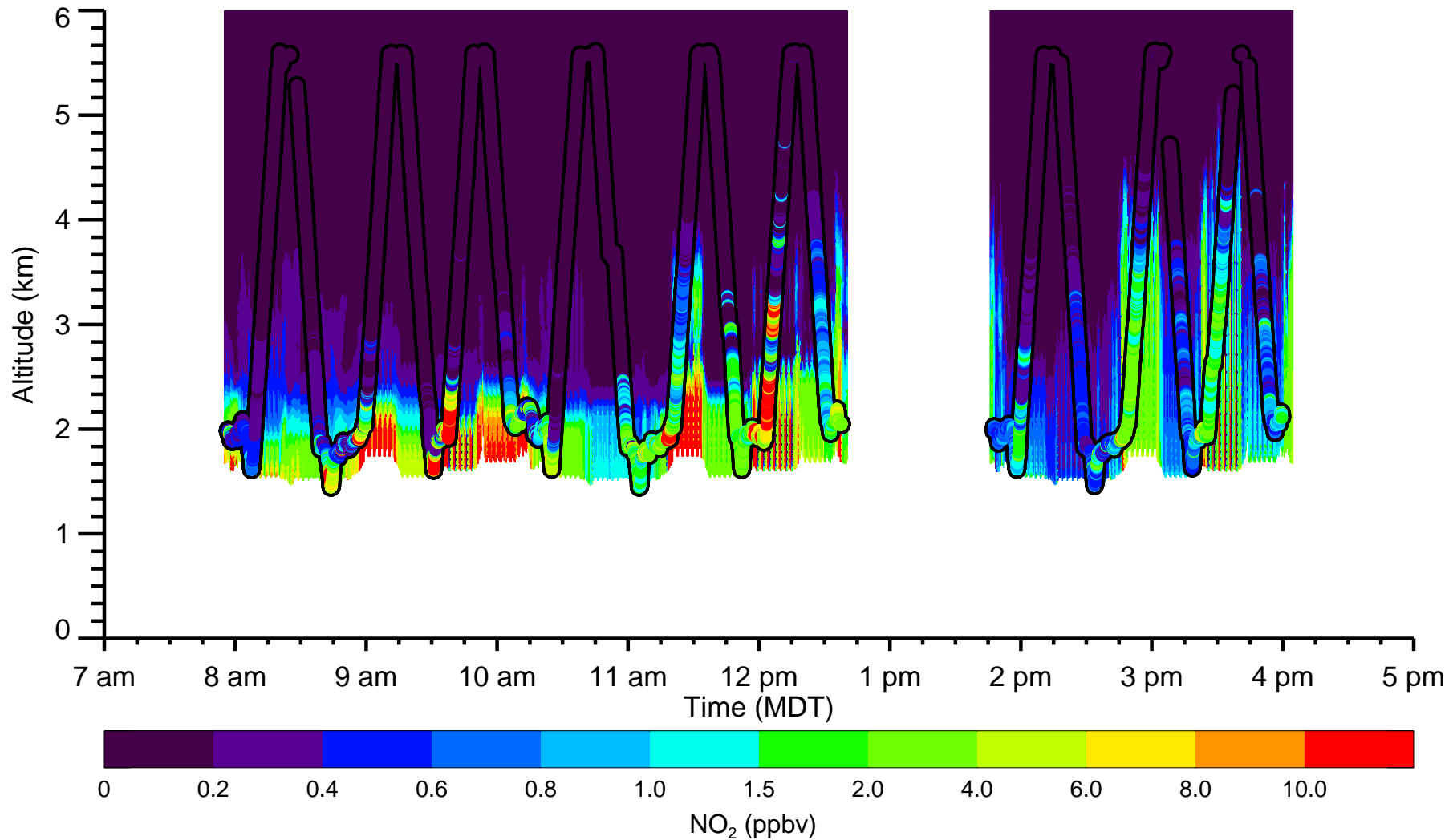
Flight #12 08/06/2014 WRFChem NO 2 and Weinheimer NO 2
