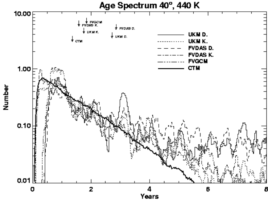
Figure 6 Same as Figure 2 for 40° release.
