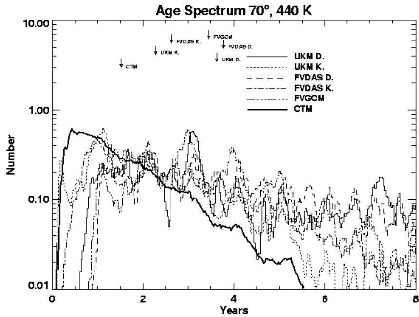
Figure 8 The age spectrum for the 70° N release experiment. See Figure 2 for details.
