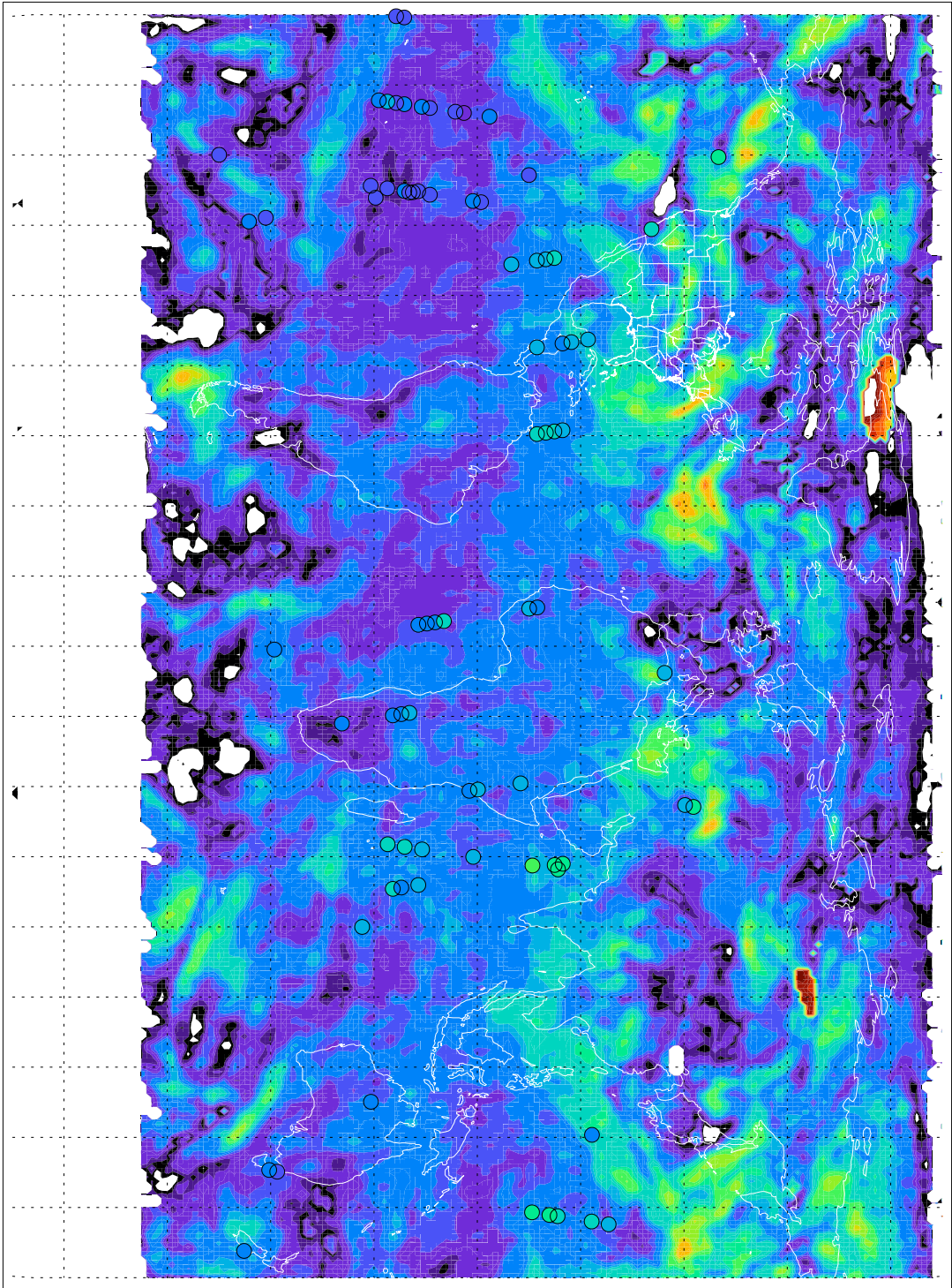
Trop. Ozone Column April 28 2005
