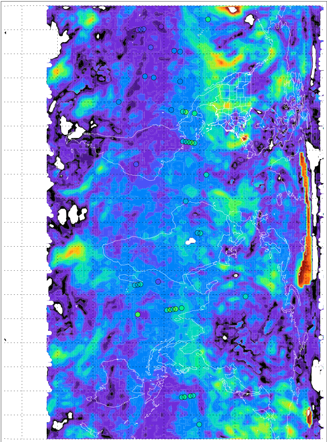
Trop. Ozone Column April 25 2005
