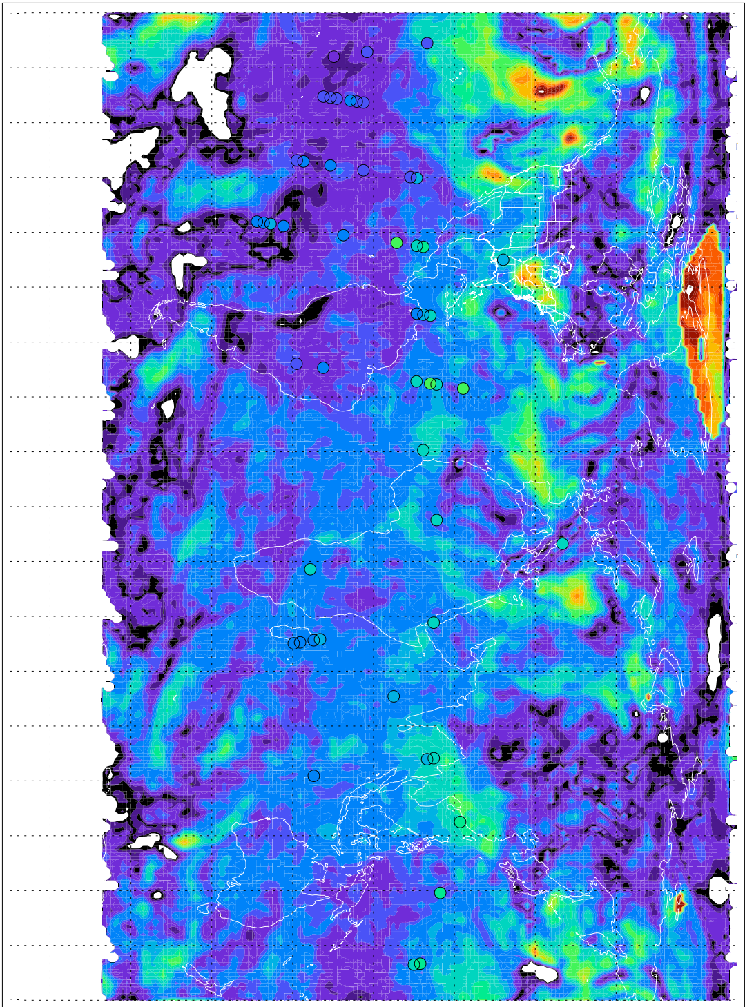
Trop. Ozone Column April 23 2005
