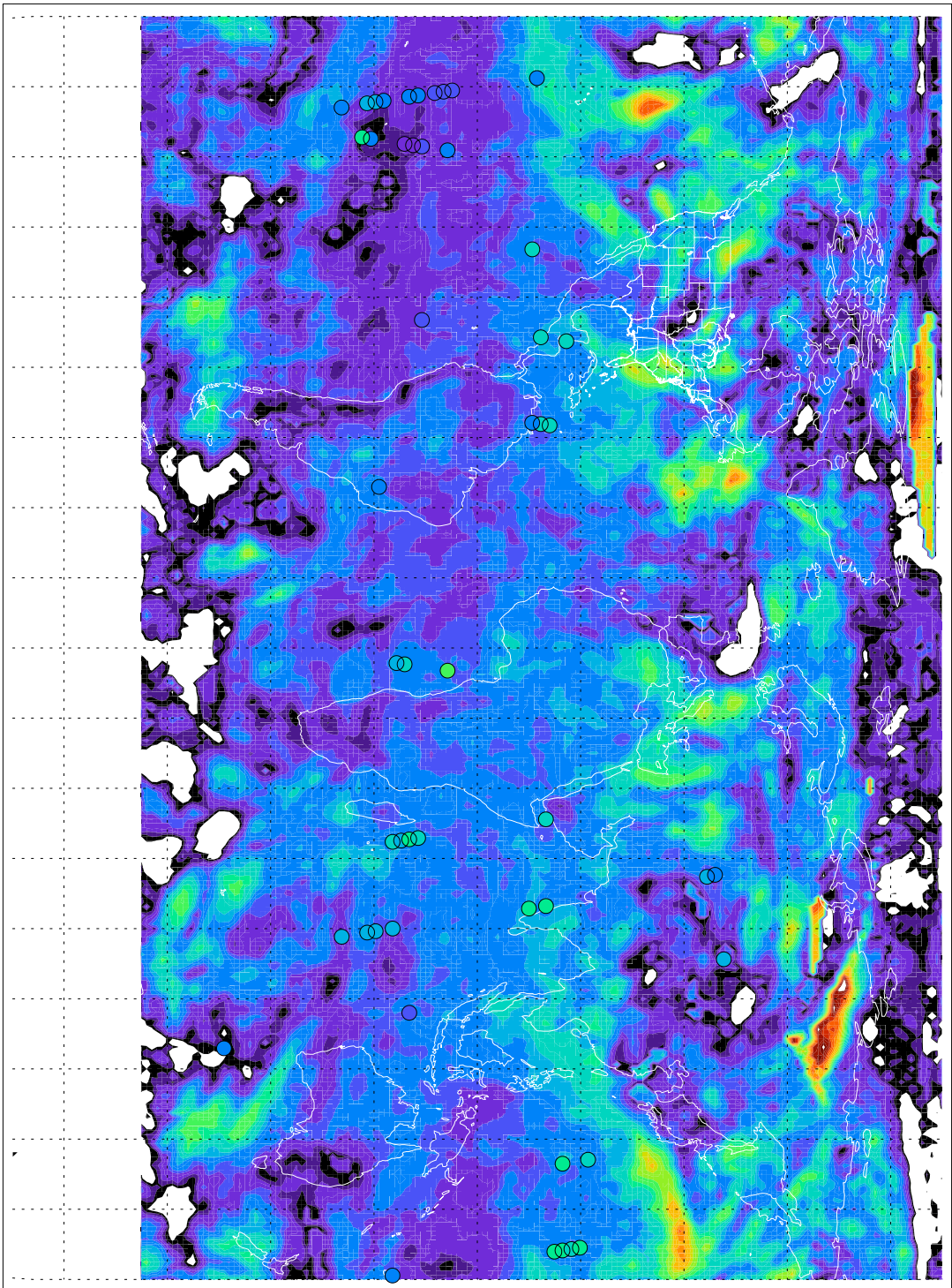
Trop. Ozone Column April 27 2005
