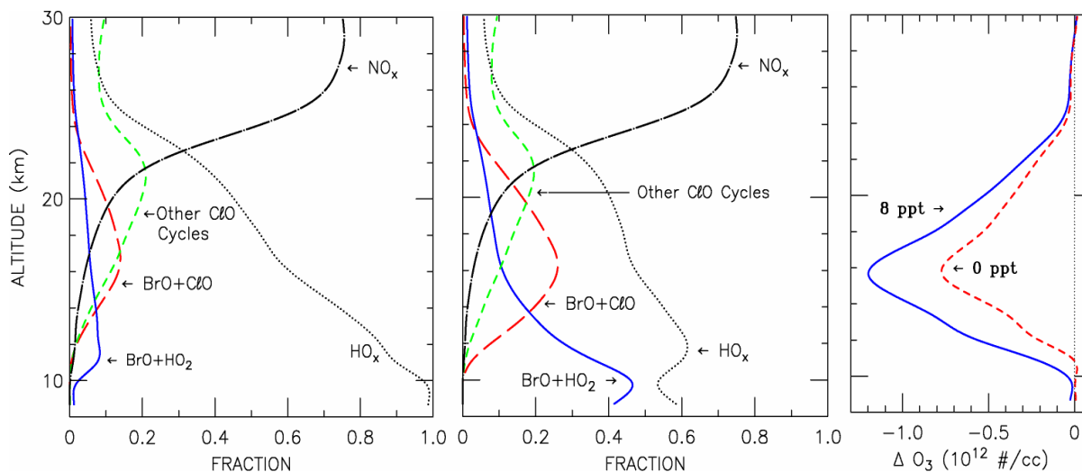
FIGURE 6.1 Ozone Photochemistry. Enhanced Bromine: Increased ozone depletion due mainly to BrO + ClO cycle. BrO + HO_2 cycle becomes a significant O_3 sink below 16 km ( BrO + HO_2 does not drive O_3 depletion if Br_y^{Trop} is constant over time).
