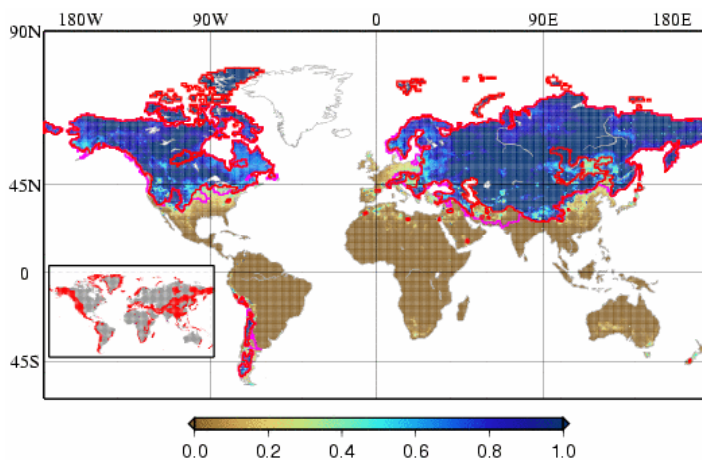
FIGURE 11.7 Accumulated annual snowfall divided by annual runoff over the global and land regions. The red lines indicate the regions where streamflow is snowmelt dominated, and where there is not adequate reservoir storage capacity to buffer shifts in the seasonal hydrograph. The pink lines indicate additional areas where water availability is predominantly influenced by snowmelt generated upstream (but runoff generated within these areas is not snowmelt dominated). The inset shows regions of the globe that have complex topography using the criterion of Adam et al. (2005).
