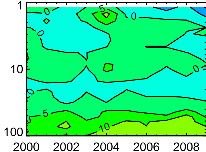
GMI CTM-Obs (%) Hohenpeiss
