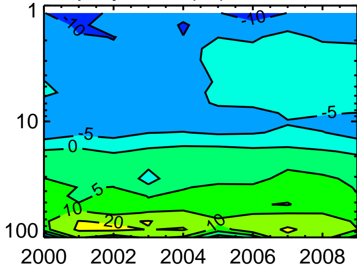
Replay-Obs (%) MaunaLoa
