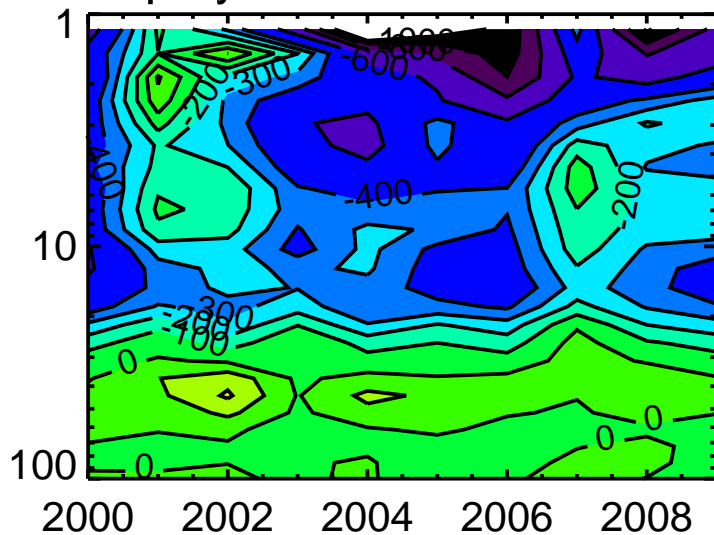
Replay-Obs HauteProvence
