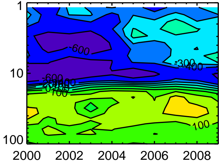
Replay-Obs MaunaLoa
