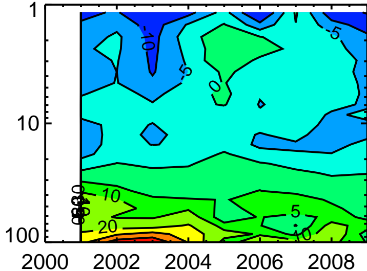
Replay-Obs (%) TableMountain
