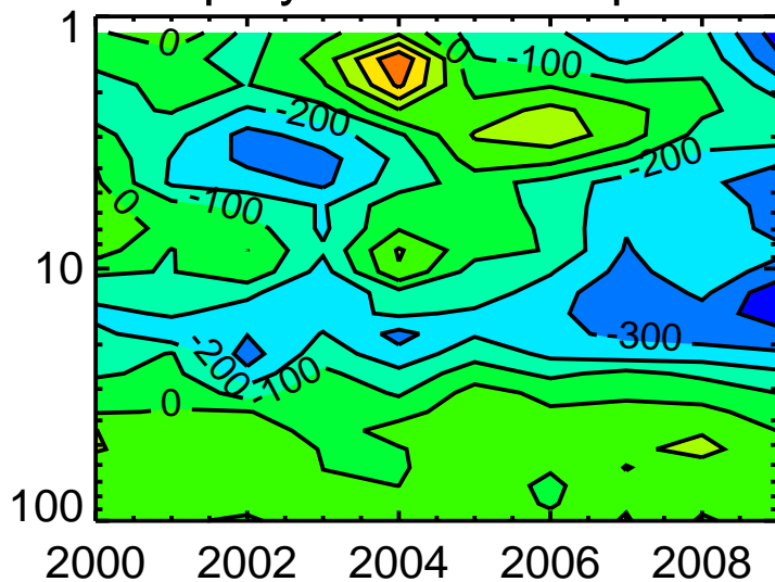
Replay-Obs Hohenpeiss
