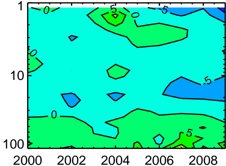
Replay-Obs (%) Hohenpeiss
