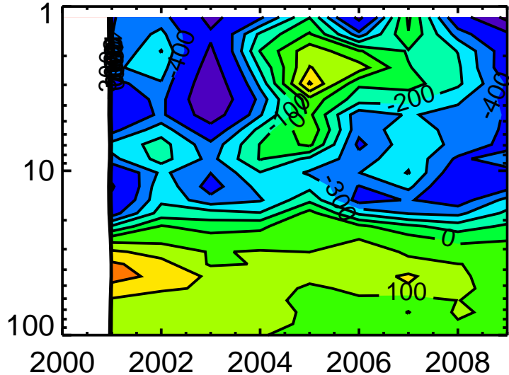
Replay-Obs TableMountain
