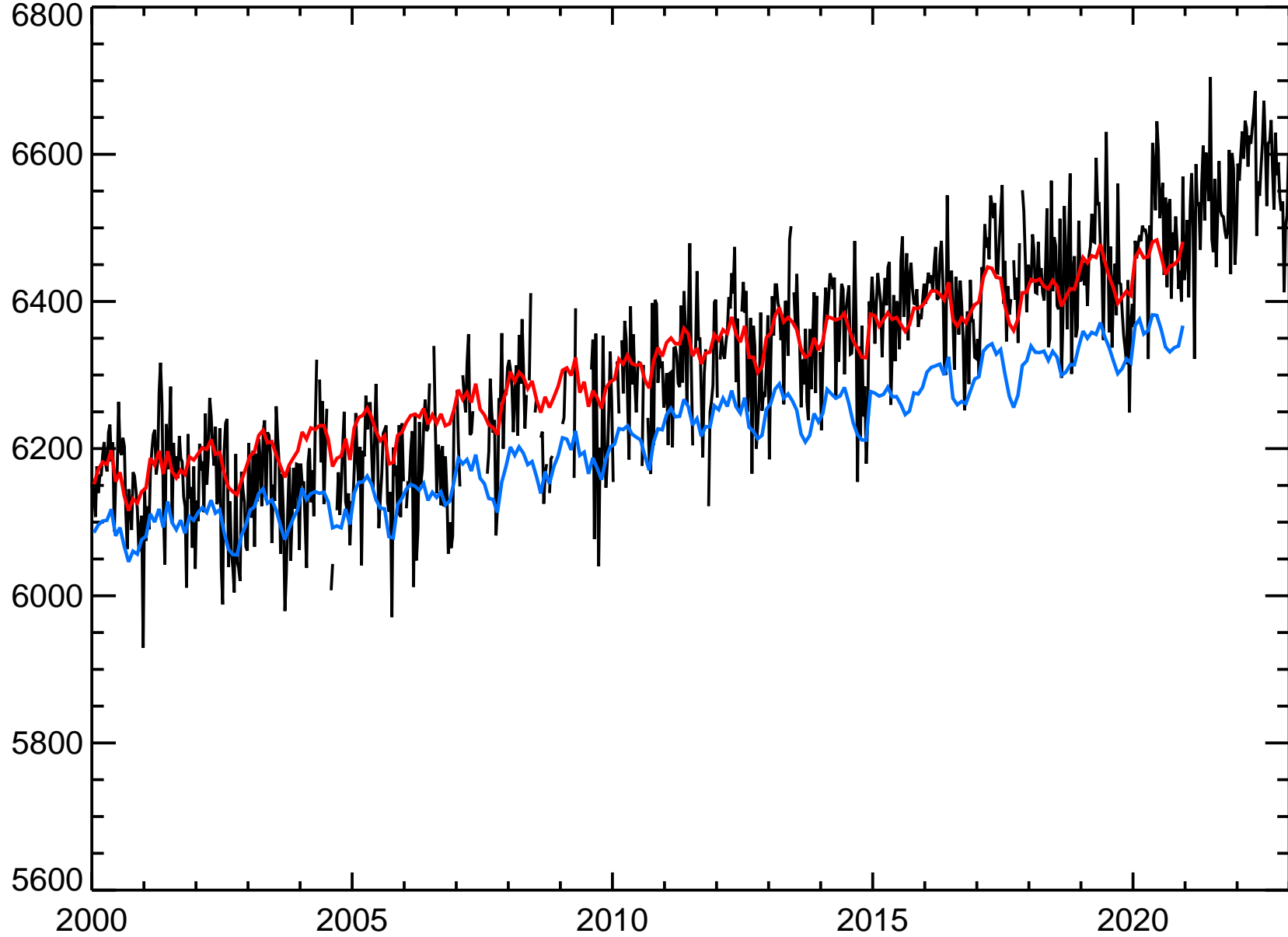
GMI CTM (blue) and Replay (red). Lauder 10-day Avg (black) Lauder Total Column N 2 O
