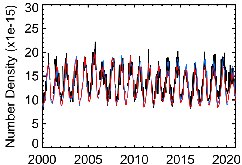
Lauder HNO 3
