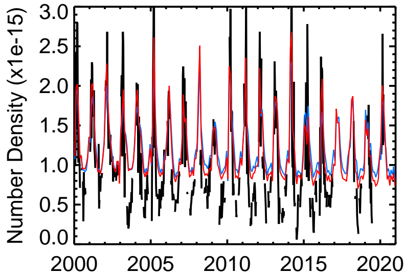
Kiruna ClONO 2
