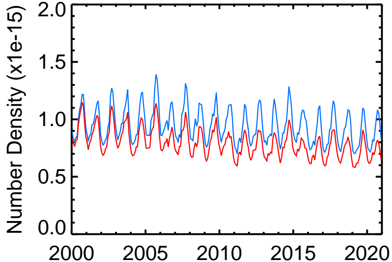
Wollongong ClONO 2
