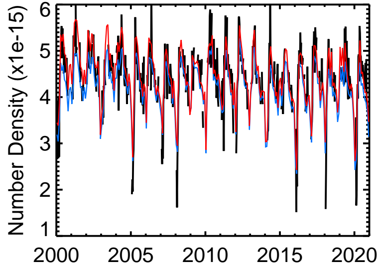
Kiruna HCl
