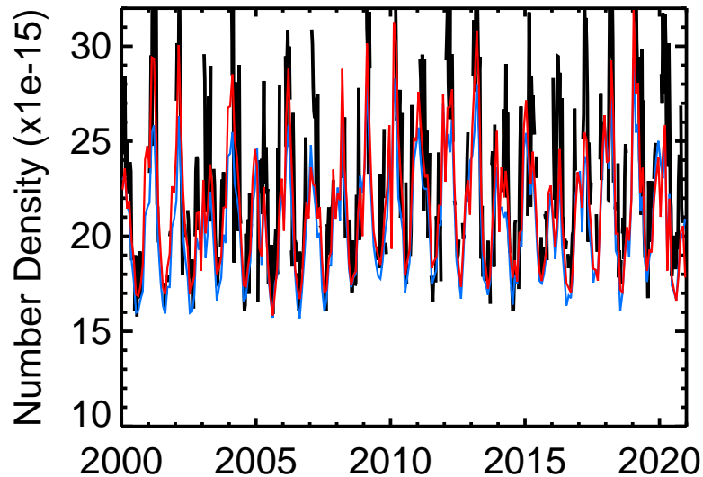
Kiruna HNO 3
