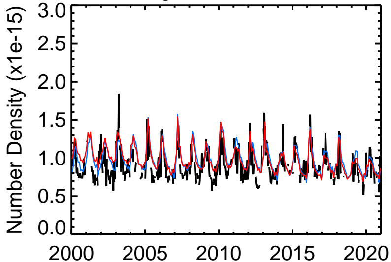
Jungfrau ClONO 2
