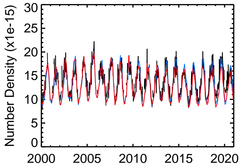
Lauder HNO 3
