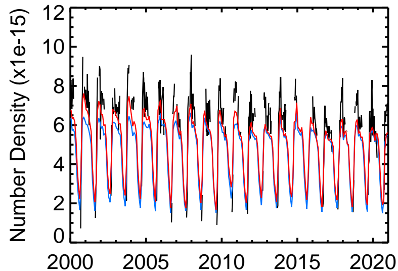
Arrival HCl
