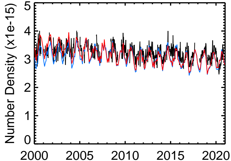
Wollongong HCl
