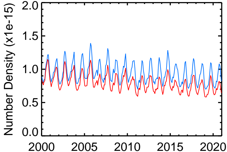
Wollongong ClONO 2
