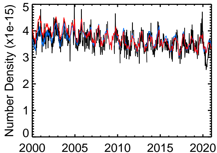
Lauder HCl
