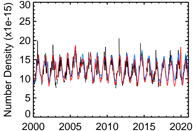
Wollongong HNO 3
