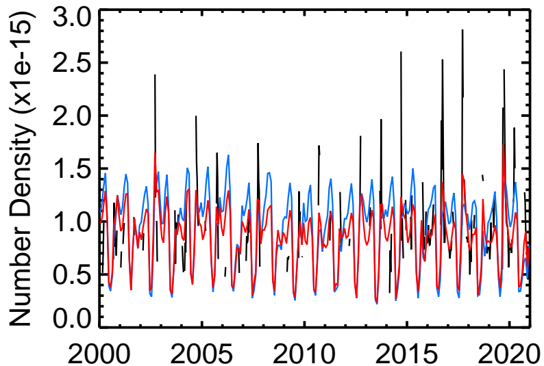
Arrival ClONO2
