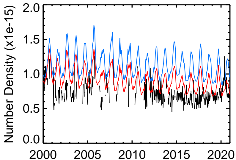
Lauder ClONO 2
