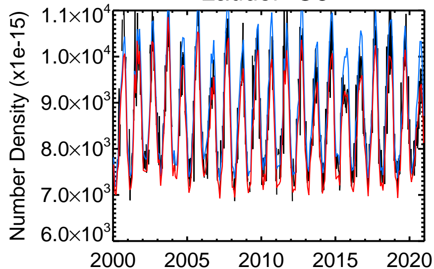
Lauder O 3
