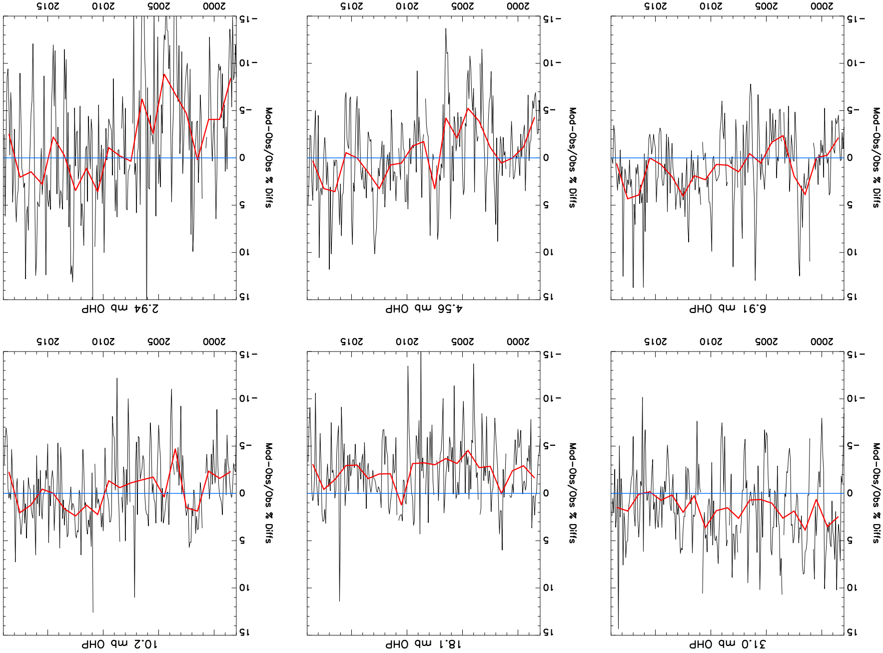
Monthly Avg O3 Differences (%), Model-OHP, 1998-2018 & Annual Mean Diff (red)
