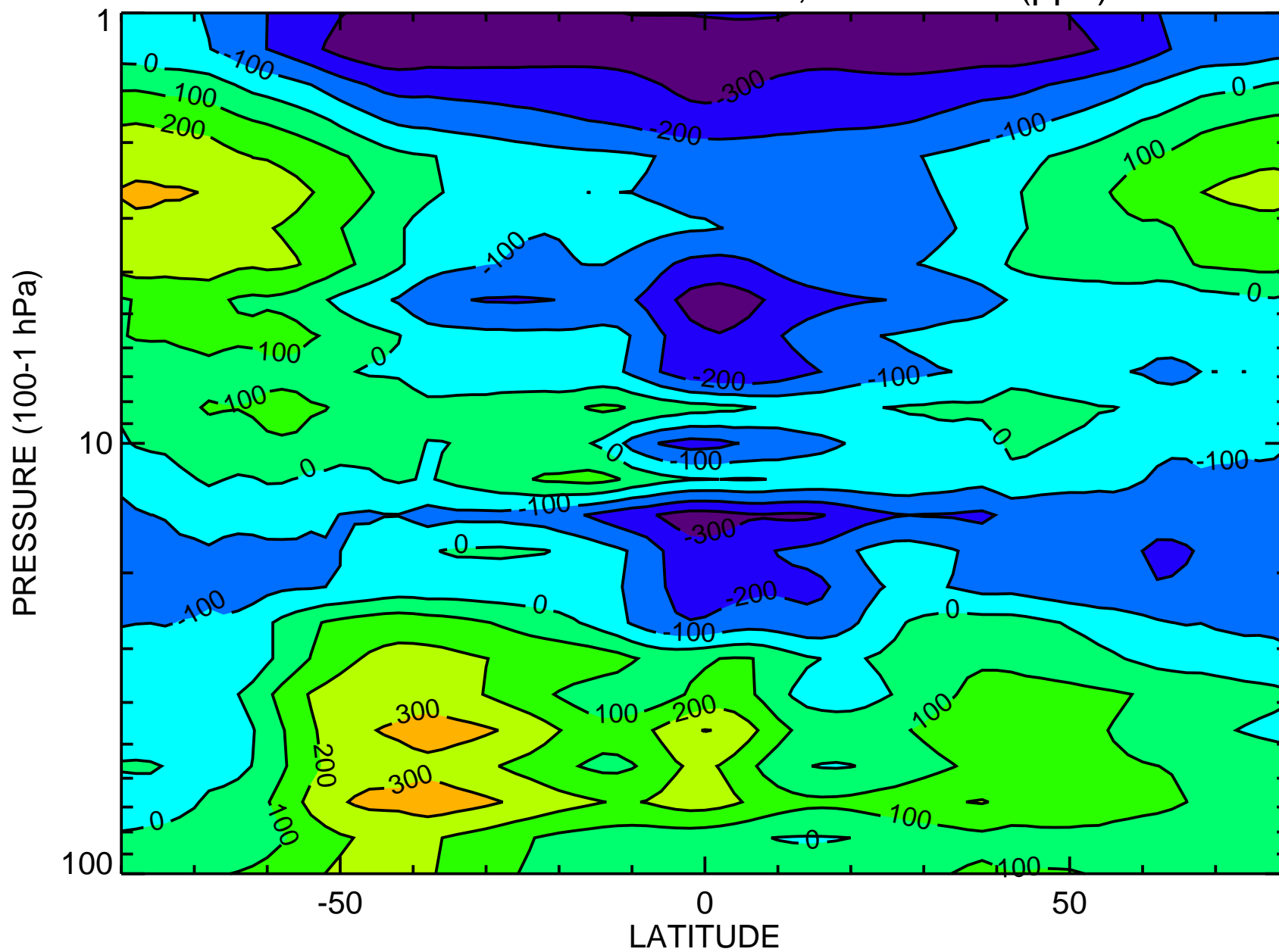
GMI - MLS Annual Mean O3, 2013-2016 (ppb)
