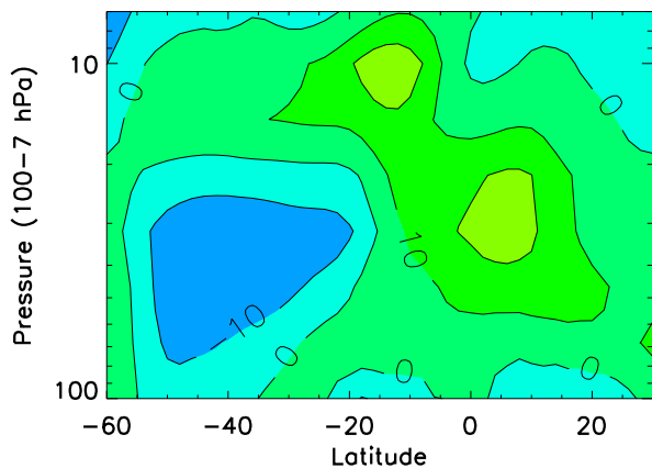
2015 HNO 3 Anom OCT
