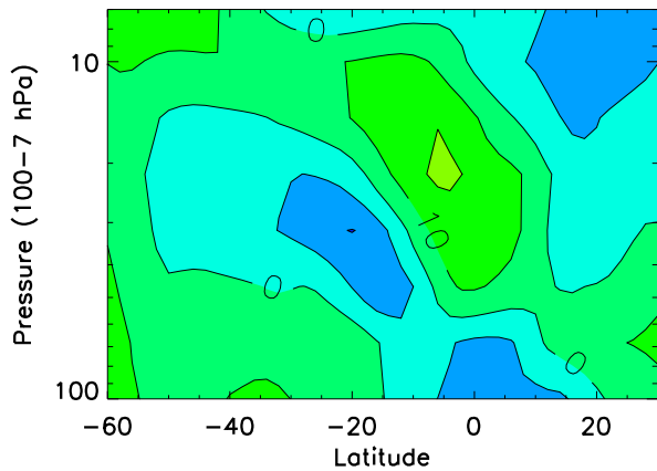
2015 HNO 3 Anom AUG
