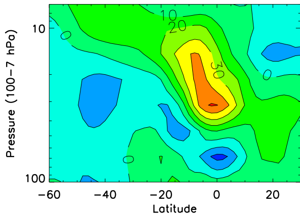
2022 HNO 3 Anom AUG
