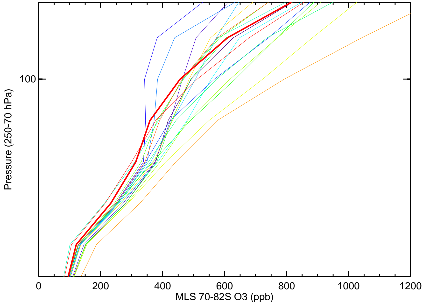
70-82S Sep ZM Daily MLS O3, 2004 (blue) - 2022 (red) SEP
