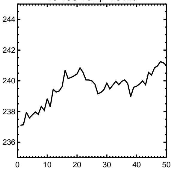
10-18S Temp 4.6 mb
