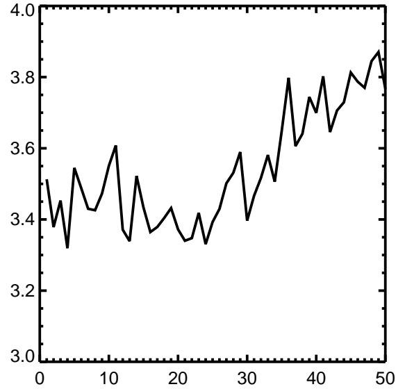
10-18S HNO 3 31 mb
