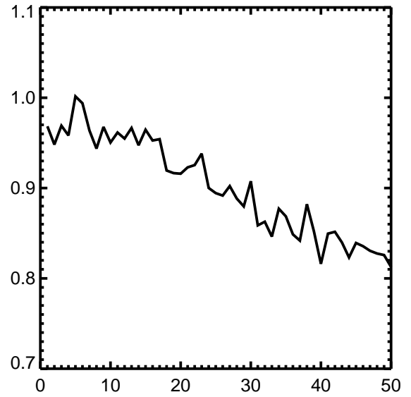
10-18S HCl 31 mb
