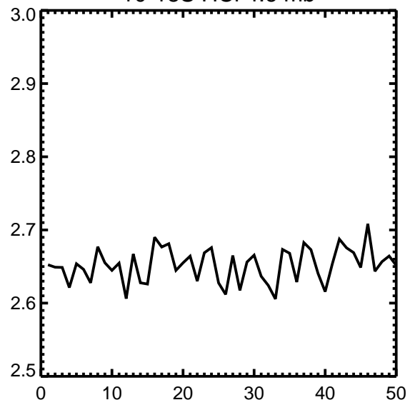
10-18S HCl 4.6 mb
