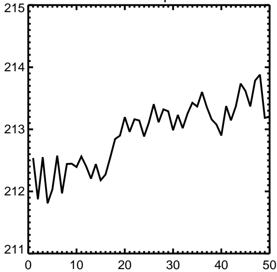
10-18S Temp 31 mb
