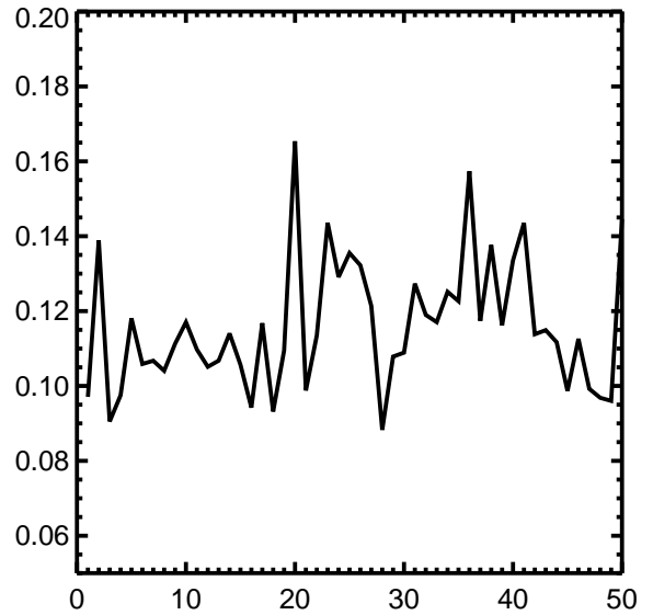
10-18S ClO 31 mb
