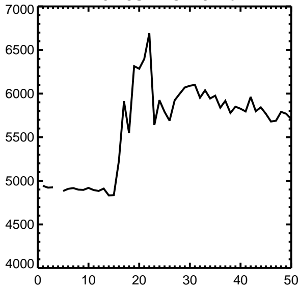
10-18S H2O 4.6 mb
