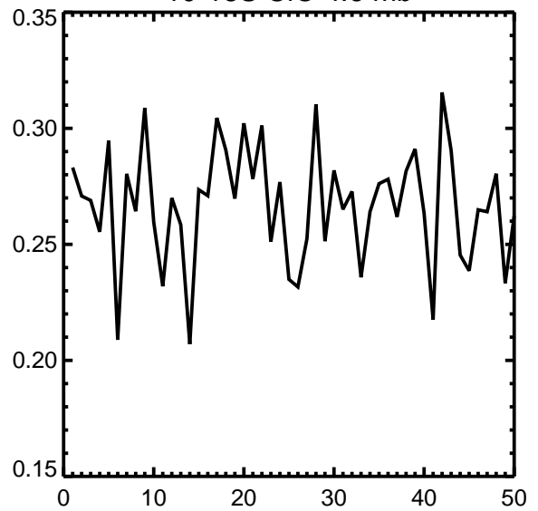
10-18S ClO 4.6 mb
