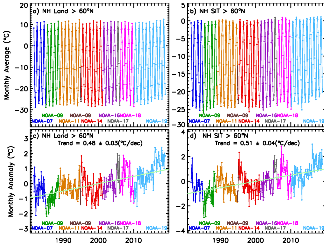
Figure 3. Plots of monthly averaged surface temperature data (>60°N) as derived from Advanced Very High Resolution Radiometer (AVHRR) over (a) land and (b) sea ice. Contributions from the AVHRR sensors from NOAA-07 to NOAA-19 are shown in different colors. Plots of monthly anomalies of surface temperatures over (c) land and (d) sea ice (SIT). The anomalies were derived from the monthly data by subtracting the climatology for each month. The trends as indicated are the result of linear regression.
