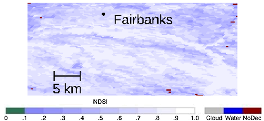
Figure 7. Terra Moderate Resolution Imaging Spectroradiometer (MODIS) Collection 6 (C6) Normalized Difference Snow Index (NDSI) snow-cover map of a 1,685-km 2 area of the boreal forest in central Alaska, acquired on 1 March 2016. The NDSI provides information that can be tuned to a specific study area to estimate fractional snow cover (FSC) in each pixel if a user has detailed information about the snow cover in their study area. The red areas represent “no decision” by the snow-mapping algorithm.
