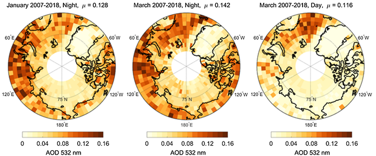
Figure 17. Mean aerosol optical depth (AOD; unitless) from the Cloud-Aerosol Lidar and Infrared Pathfinder Satellite Observation (CALIPSO) satellite for (left) January during night, (center) March during night, and (right) March during day. The mean data are for “all-sky” conditions and averaged from 2007 to 2018. CALIPSO does not detect AOD values below a detection threshold, so the mean AOD is biased to higher AOD events in spatial and temporal averages. It has lower detection sensitivity in daylight, only detecting the strongest Arctic aerosol events (center and right). Consequently, the daytime data are systematically biased low (Di Pierro et al., 2013). CALIPSO’s detection sensitivity is lowest in summer, which leads to a large low bias (not shown) that is compounded by the fact that AOD values tend to be seasonally lowest in summer. There are missing data over the pole because the instrument is on a satellite in sun-synchronous orbit and because of instrument design.
