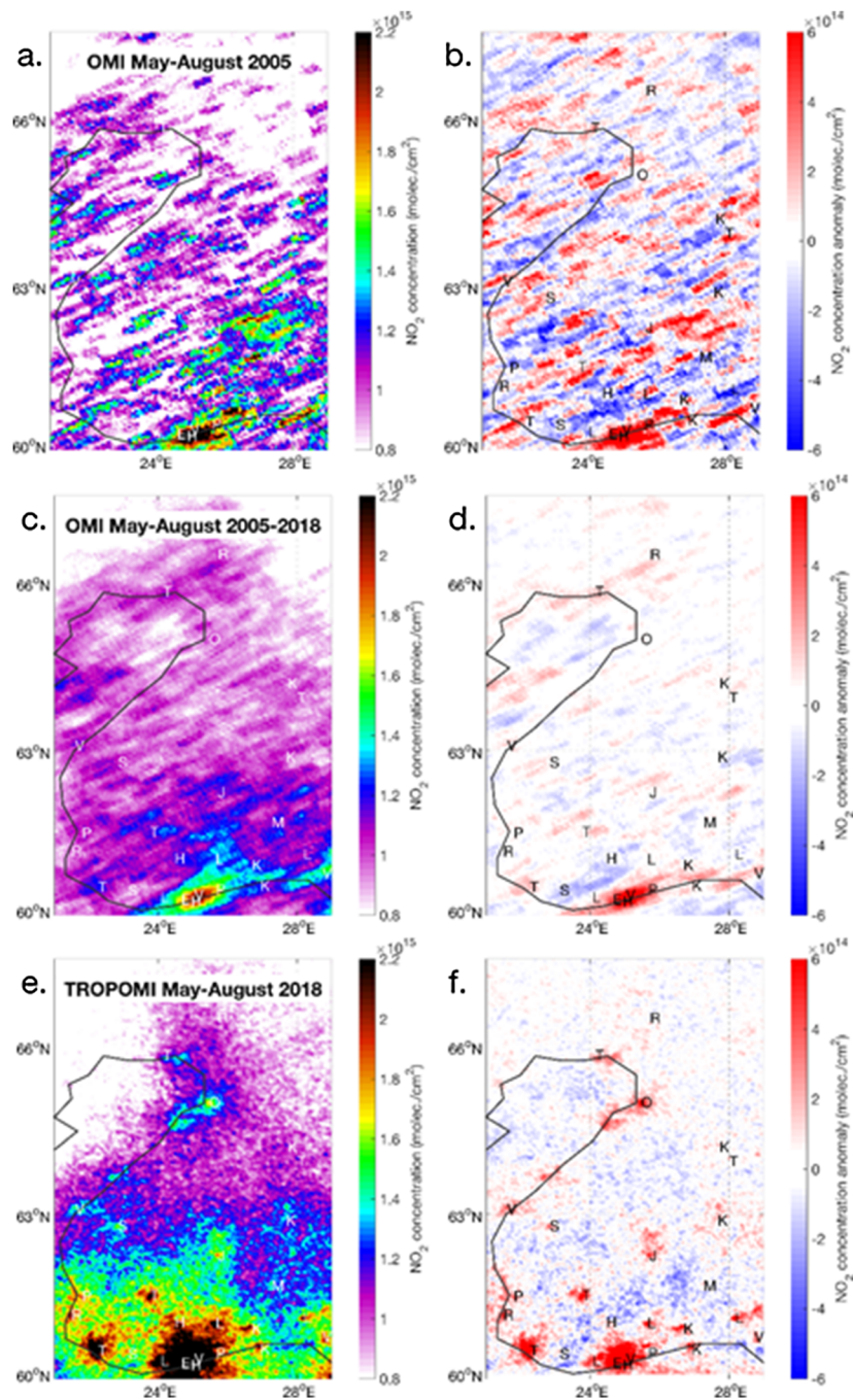
Figure 16. (a) Ozone Monitoring Instrument (OMI) \text{NO}_2 data (molecules/ \text{cm}^2 ) for May–August 2005 over Finland at 0.05^\circ latitude \times 0.05^\circ longitude resolution. The data were filtered by wind speed ( <5 m/s) to minimize the effect of dispersion. The letters correspond to the locations of cities. Because of relatively low signal-to-noise, the data are noisy. (b) To improve the detectability of small sources, the average signal of surrounding pixels ( 1^\circ latitude \times 1^\circ longitude) is removed from every grid pixel so that red pixels correspond to \text{NO}_2 levels larger than the local background. This procedure leads to the small cities around Helsinki, the largest source in Finland, to appear below background levels. (c and d) The same as the top row, but as the average of May–August 2005–2018. The average of multiple years reduces noise, allowing smaller sources to become apparent. (e and f) The same as the top row but using TROPOMI \text{NO}_2 tropospheric columns averaged over the period May–August 2018 at 0.02^\circ latitude \times 0.02^\circ longitude resolution. TROPOMI smaller pixels and higher signal-to-noise ratio improve the detection of emission sources (cities).
