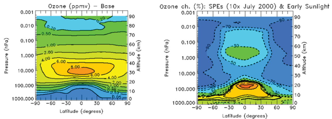
Figure 5. The 2D map of atmospheric ozone destruction driven by XUV flux from an active star and a 10xJuly 2000 SEP event (right panel, Model D) with respect to the base model (left panel; Model A).
